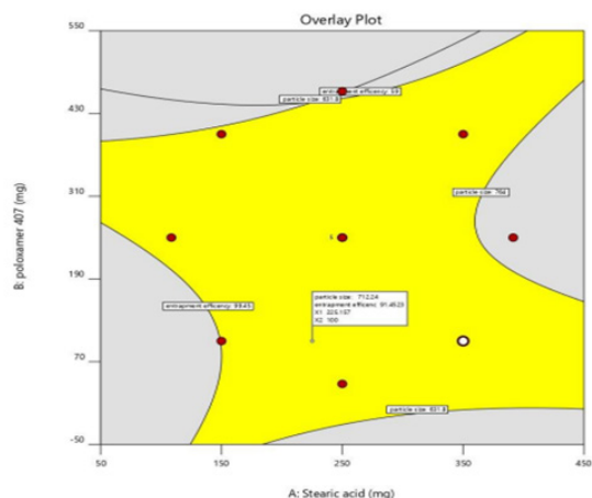
Figure 5: Overlay plot of optimized formula.
