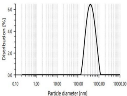
Figure 6: Particle size analysis.
