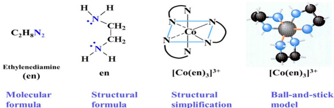
Figure 8: Structure diagrams of ethylenediamine ligands and their complexes.
